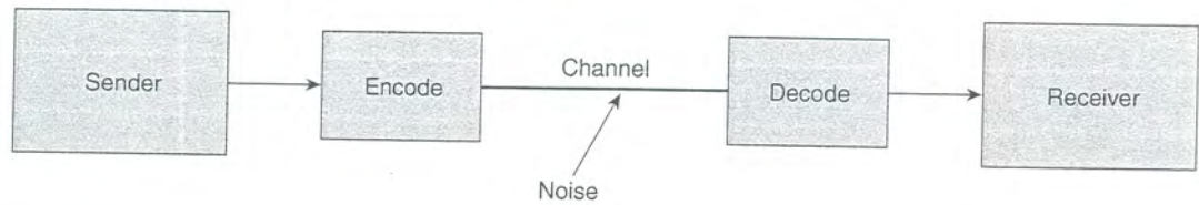
FIGURE 1-3 Information-Communication Model
