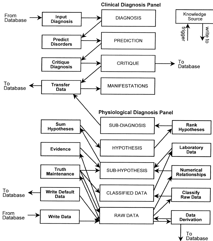
Fig. 2. Implementation of the blackboard model of problem solving in the KBS prototype (from Chelsom, 1990).
