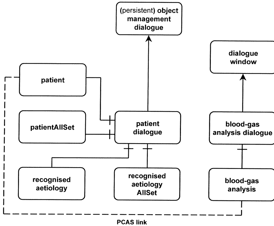
Fig. 7. Class diagram of the patient data dialogue object structure created by the OMS module.
