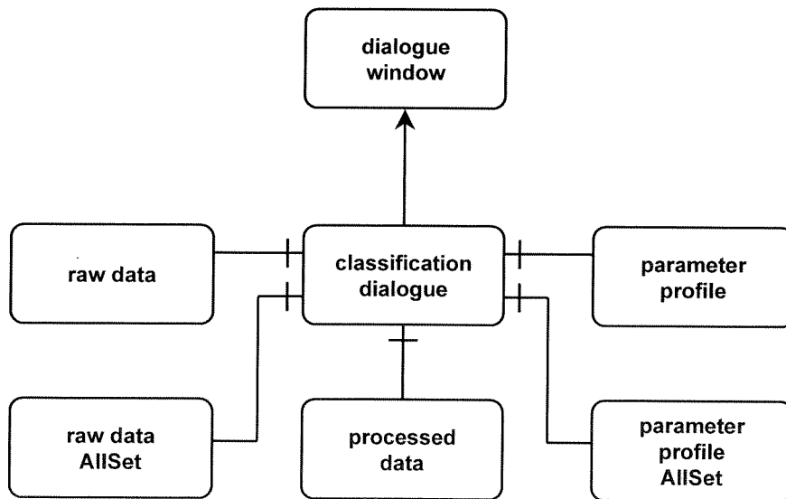
Fig. 8. Class diagram of data classification dialogues
