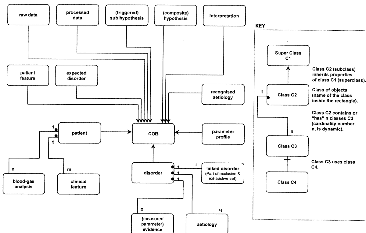
Fig. 4. Class diagram of the models used by the ICIMS system OMS module for the derivation of the persistent object structures required to support the management of the clinical information generated in the process of monitoring the ICU patient, the knowledge base utilised for the interpretation of the acquired clinical information, and the blackboard objects required to support the application of the prototype task-domain model.
