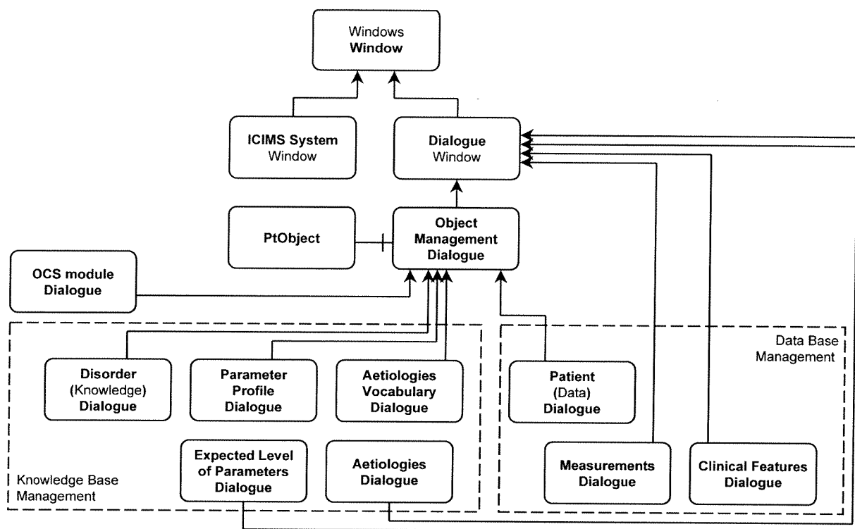
Fig. 5. Class structure diagram linking the ICIMS system COB to the OMS module, for the acquisition, review and update of the data and knowledge model derived objects.
