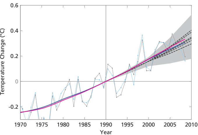
Figure 3 Changes in global average surface air temperature (smoothed over 11 years) relative to 1990. The blue line represents data from Hadley Center (UK Meteorological Office); the red line is GISS (NASA Goddard Institute for Space Studies, USA) data. The broken lines are projections from the IPCC Third Assessment Report, with the shading indicating the uncertainties around the projections 3 (data from 2007 and 2008 added by Rahmstorf, S.).
