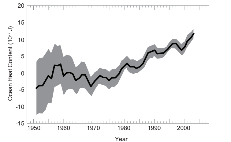
Figure 4 Change in ocean heat content since 1951 (observations - black line) with uncertainties (in grey shading), relative to the ocean heat content in 1961 4 .
