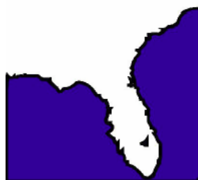
Florida w/o WAIS+GIS
