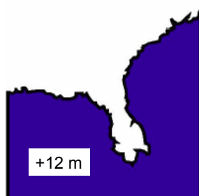
Florida w/o WAIS+GIS
