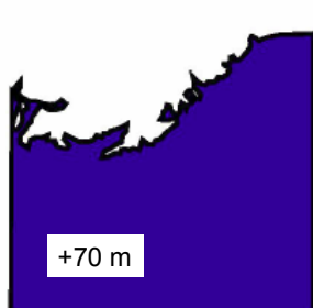
Florida w/o WAIS+GIS+EAIS
